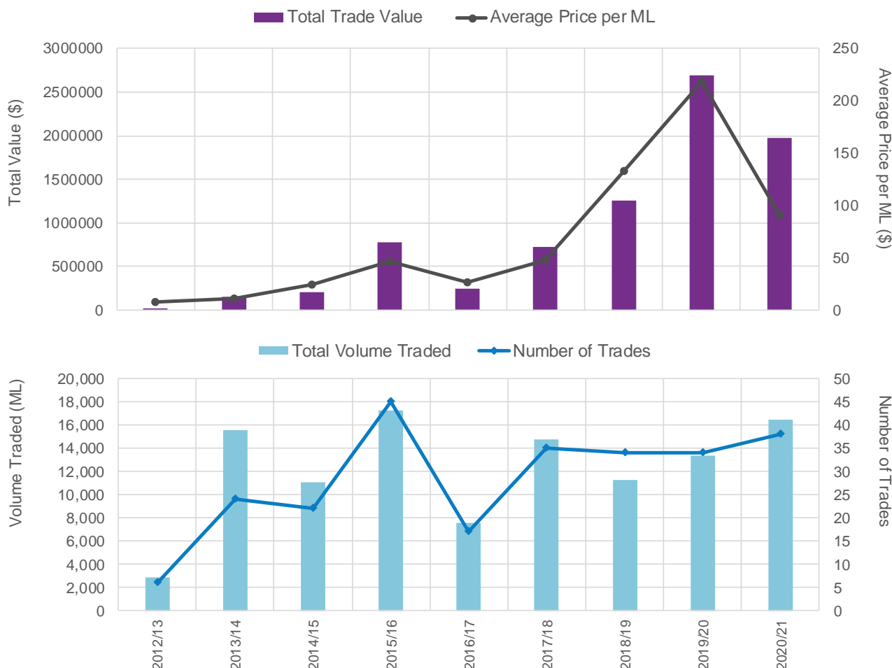
Figure 3: Lower Lachlan Groundwater Source temporary trade statistics
