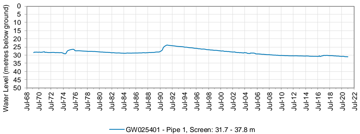
Figure 7: Hydrograph of GW025401
