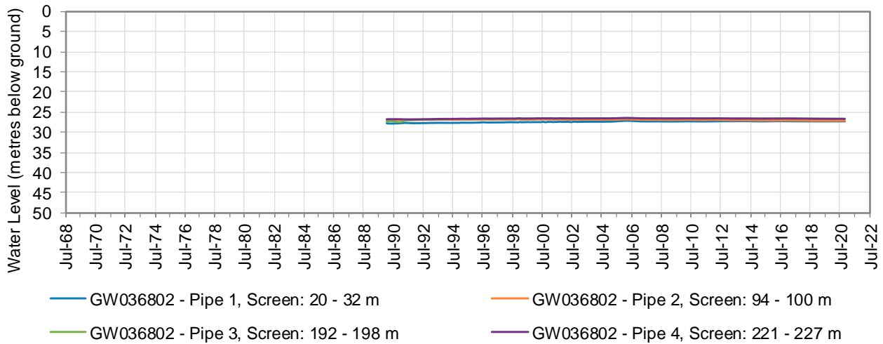
Figure 14: Hydrograph of GW036802
