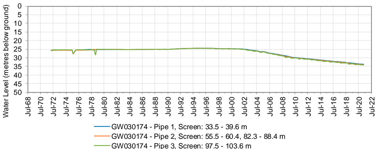
Figure 10: Hydrograph of GW030174
