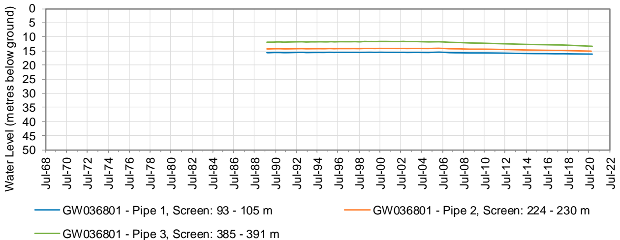
Figure 13: Hydrograph of GW036801
