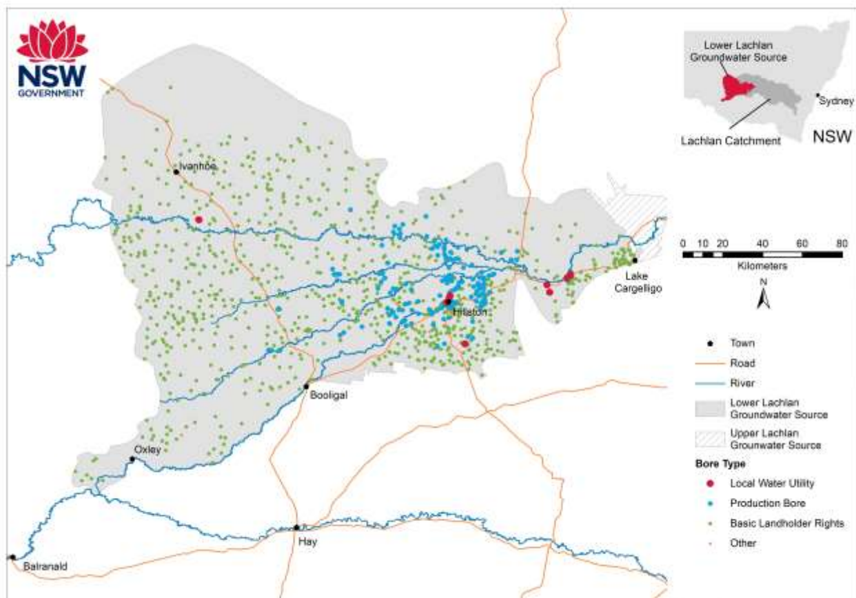
Figure 4: Lower Lachlan Groundwater Source registered bores
