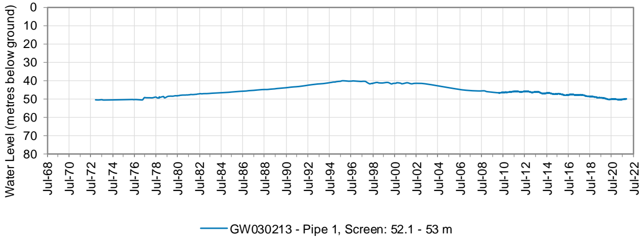
Figure 17: Hydrograph for monitoring bore GW800232 (Zone 2)
