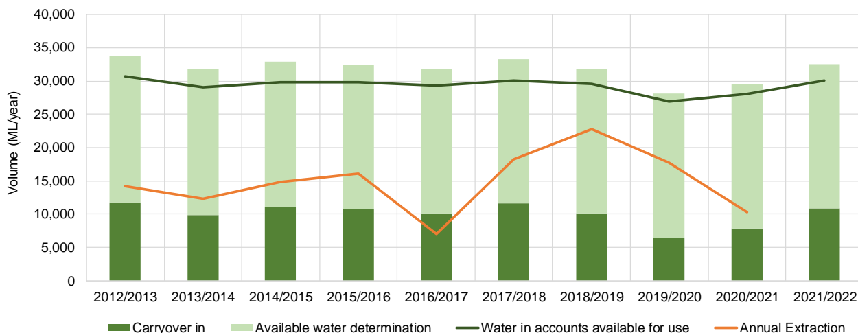
Figure 3: Account water availability and usage summary for Lower Macquarie Zone 2 Groundwater Source
