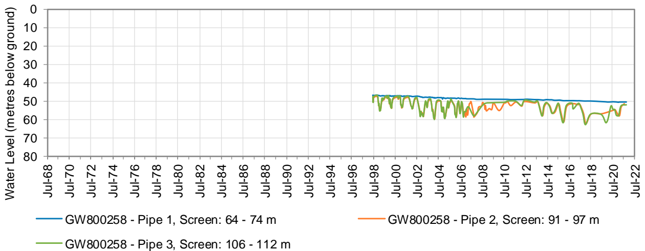
Figure 18: Hydrograph for monitoring bore GW800258 (Zone 2)
