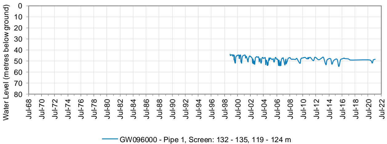
Figure 20: Hydrograph for monitoring bore GW096000 (Zone 2)
