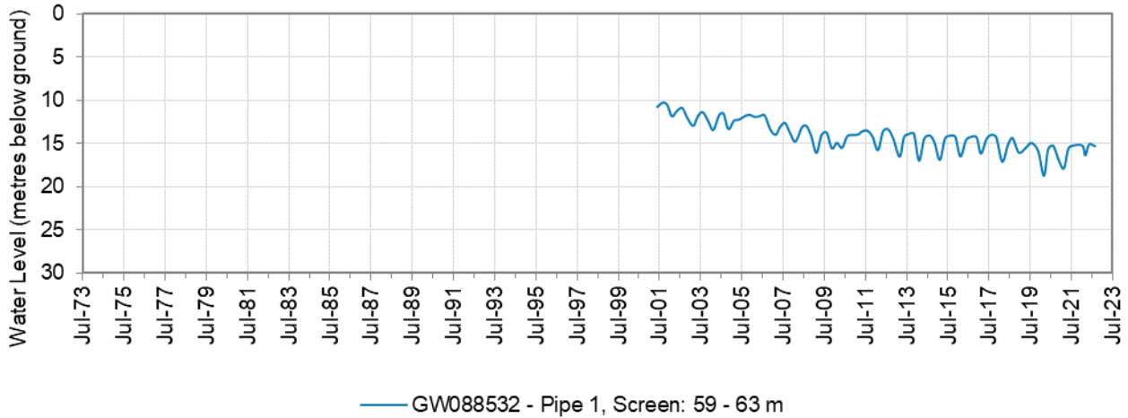
Figure 10: Hydrograph of monitoring bore GW088532
