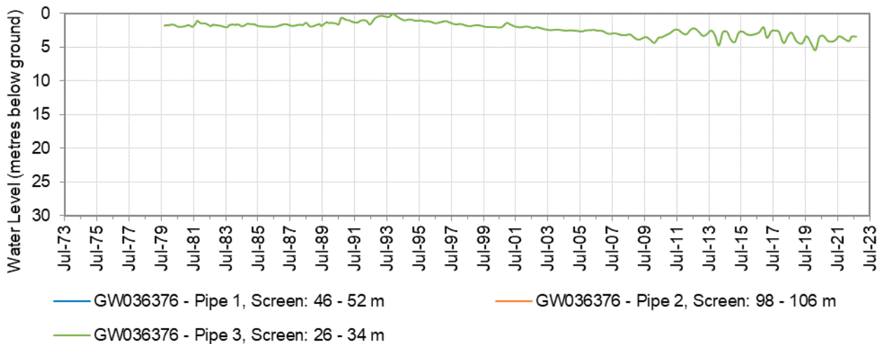
Figure 11: Hydrograph of monitoring bore GW036376
