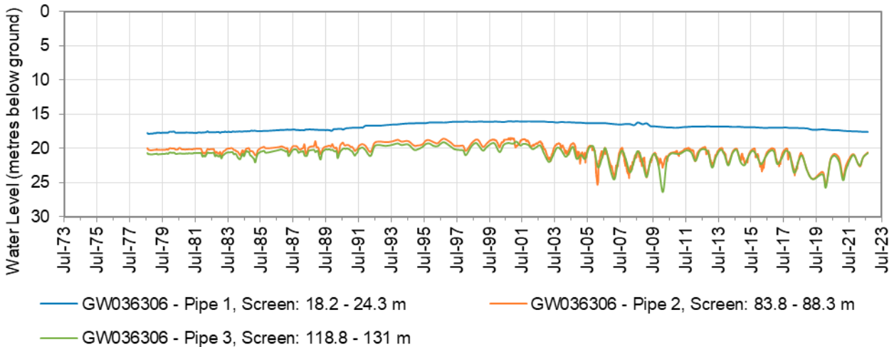
Figure 8: Hydrograph for monitoring bore GW036306
