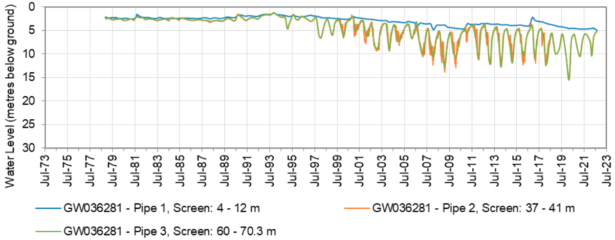
Figure 9: Hydrograph of monitoring bore GW036281
